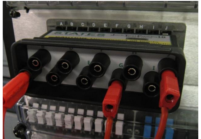
Replaceable Isolator Kit Part No. TP750
